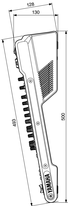
Unit: mm This illustration shows the MG20XU.
